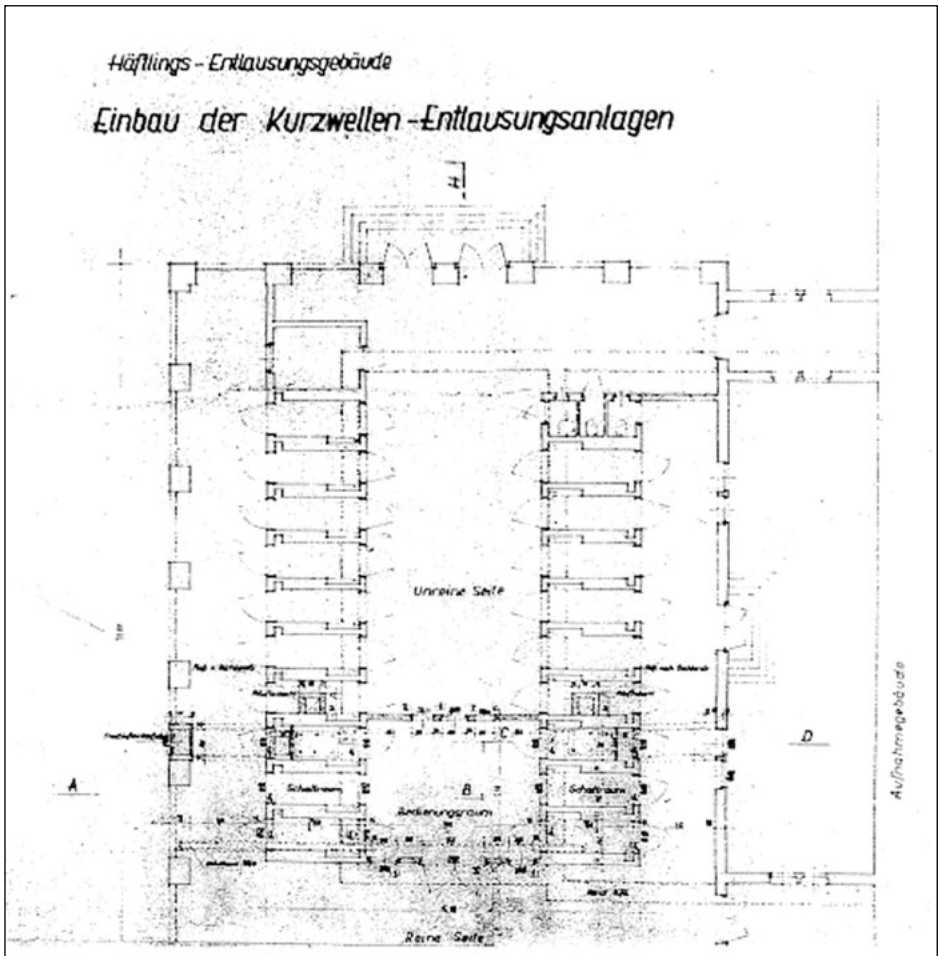
Illustration 5: German blueprint for the installation of the microwave disinfection device in the reception building of the Auschwitz Main Camp. (Russian War Archives, 502-2-149, no page number assigned)
