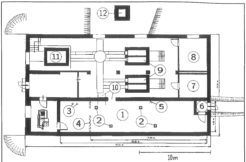
Illustration 8: Floor plan of Crematorium I at Auschwitz I/Main Camp today, after postwar alterations (“reconstruction”), following Pressac (1989: 159); taken from, Rudolf (2011: 76); numbers added as follows: 1: “gas chamber”; 2: postwar-made Zyklon B introduction holes; 3: toilet drains; 4: former partition morgue-washroom; 5: ventilation chimney of former air raid shelter; 6: air lock, today referred to as victims’ entryway; 7: urns, 8: coke; 9: badly reconstructed cremation furnaces; 10: postwar-added entry to furnace room; dotted lines: location of original entry; 11: remains of former third furnace; 12: postwar-constructed, detached chimney.
