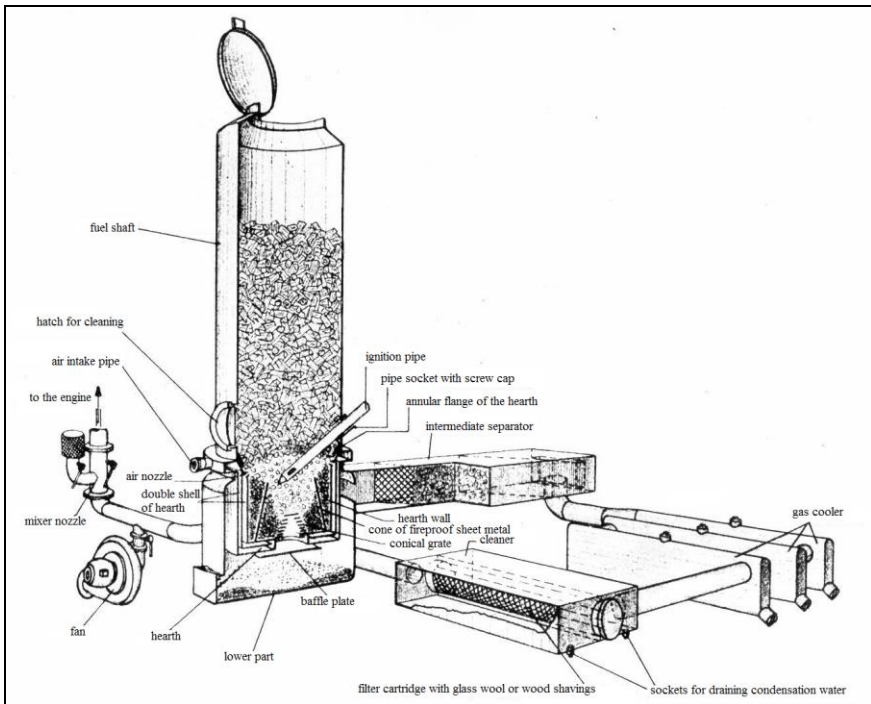
Illustration 11: Design of an Ostmark producer gas generator. (Rudolf 2003, p. 464; descriptions translated)
