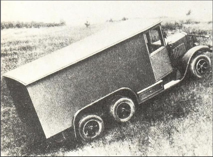
Illustration 22: Krupp L3H63 (picture from Milsom 1975, p. 104). Milsom does not give any indication as to the Sd.-Kfz. number assigned to this vehicle nor about its purpose or technical data. Since the vehicle did not seem to have had any special equipment, this might just have been a closed transportation van.
