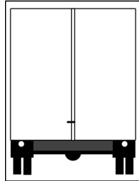
Illustration 8: Schematic drawing of rear view of the same truck with furniture cargo box, 2.30 m wide, 2.70 m high.
