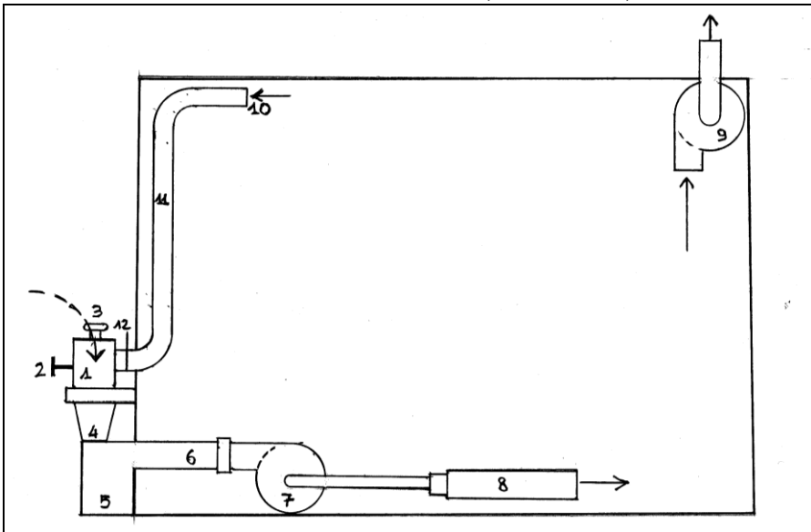
Document 5: Functional schematic of the technical equipment of the delousing chamber at Sachsenhausen. © Carlo Mattoigno.
