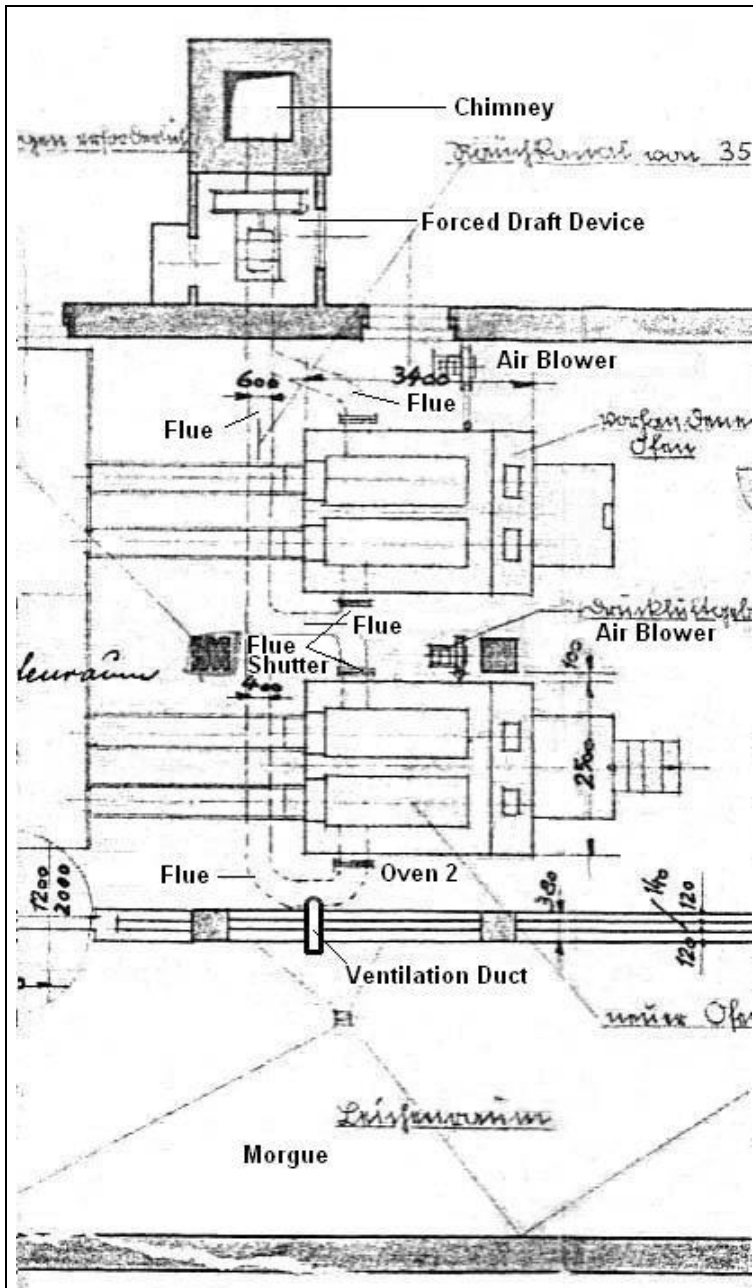
Document 10: Author's schematic drawing of first, makeshift ventilation installation for morgue of Crematorium I at Auschwitz, horizontal section, drawn onto Topf drawing D 57999, dated November 30, 1940, with English labels added.
